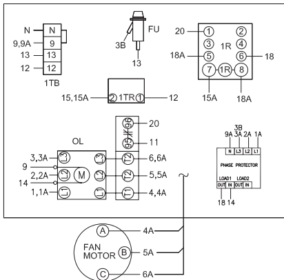
CONNECTION DIAGRAM
