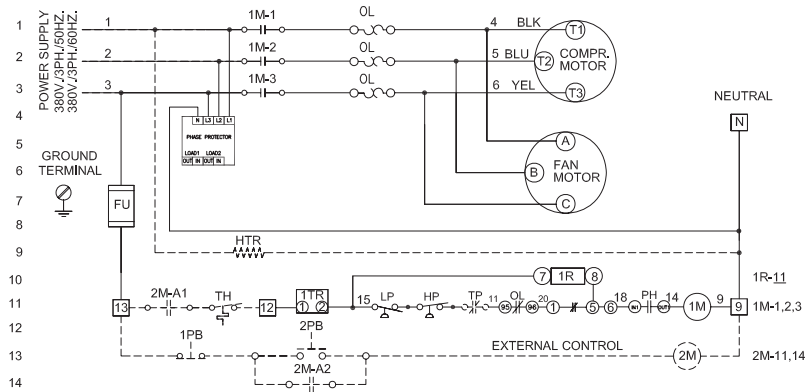
CONNECTION DIAGRAM
